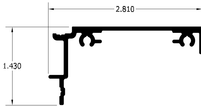
Series 3 Single Face Access Body Part #1291
